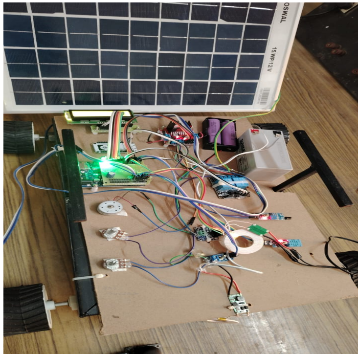
Eco-Friendly Wireless Charging With Solar Integration
