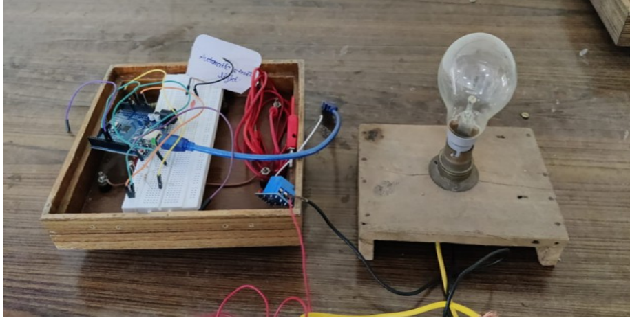
AUTOMATIC STREET LIGHT CONTROL
