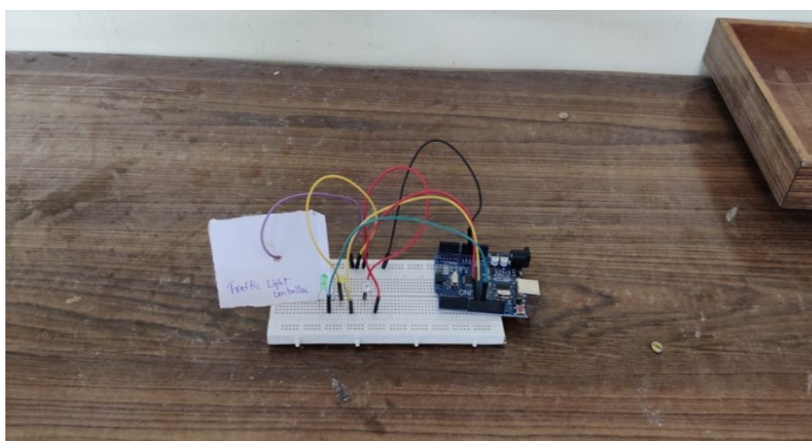
TRAFFIC LIGHT CONTROL
